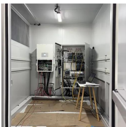
IP55 Outdoor Cabinet with Battery Compartment and Air Conditioner 24u
